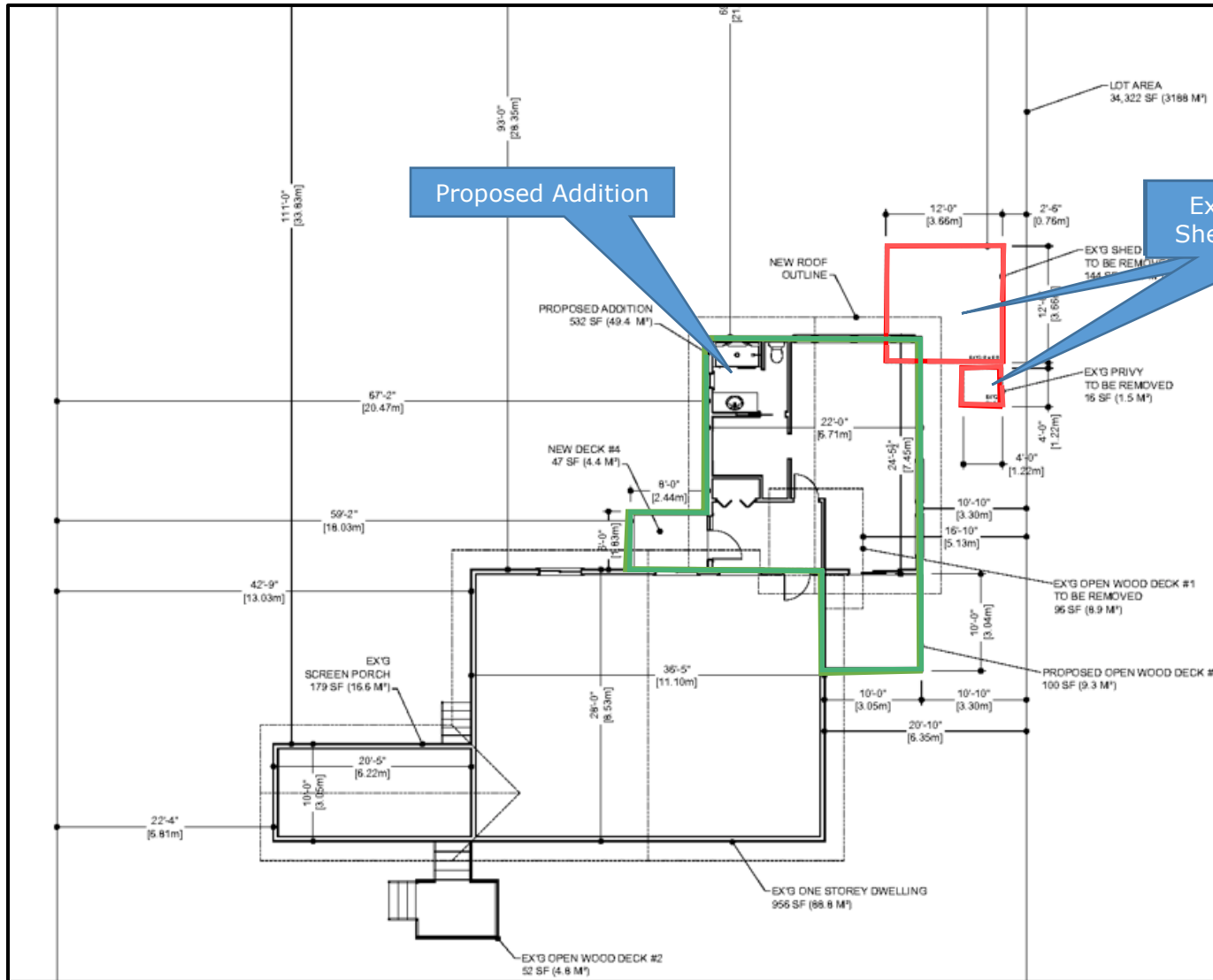
Figure 2: Proposed Site Plan (excerpt)
